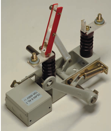
Locking device, arm and auxiliary contacts fitted on OJON 1-10/630/E1 disconnecter.
